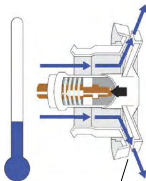
Valve closed
