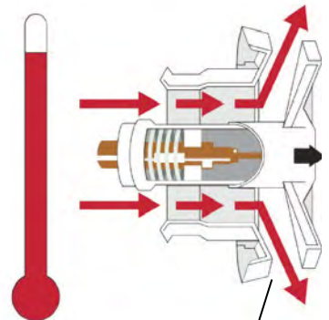
Valve open
