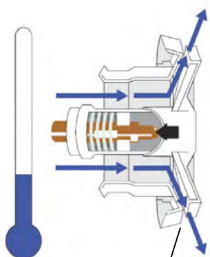
Valve closed
